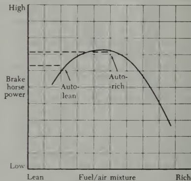
FIGURE 10-34. Power versus fuel/air mixture curve.
